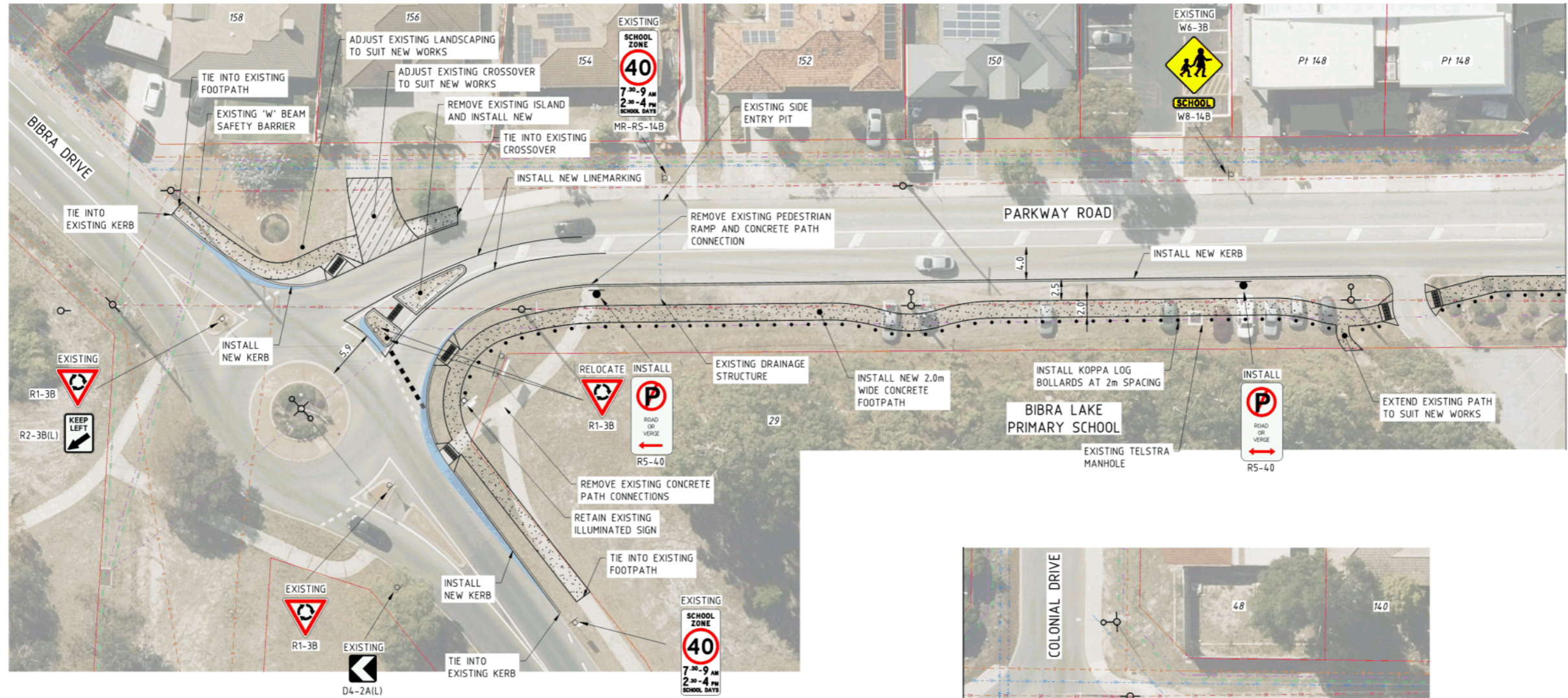
PLAN SCALE 1:250
