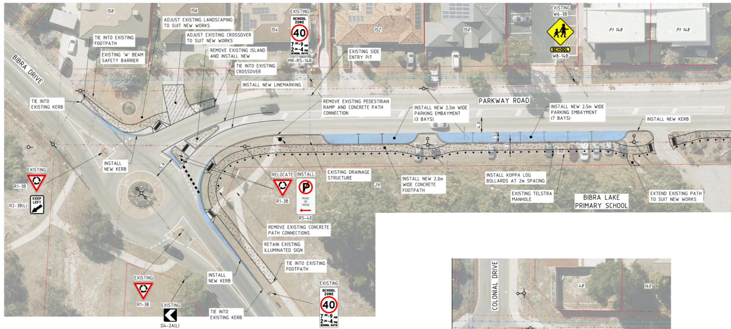
PLAN SCALE 1:250
