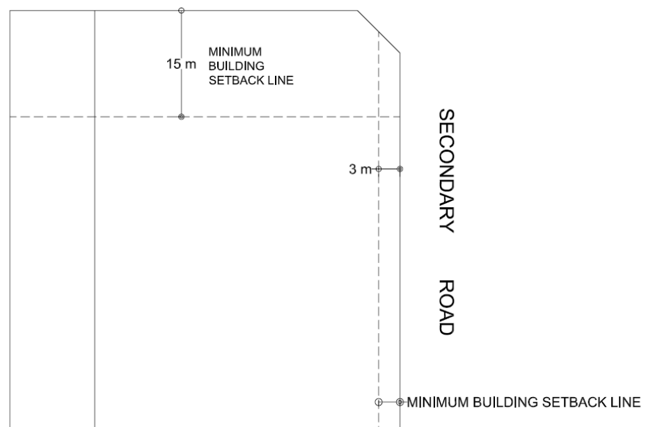
Figure 2 - Setbacks PRIMARY ROAD
